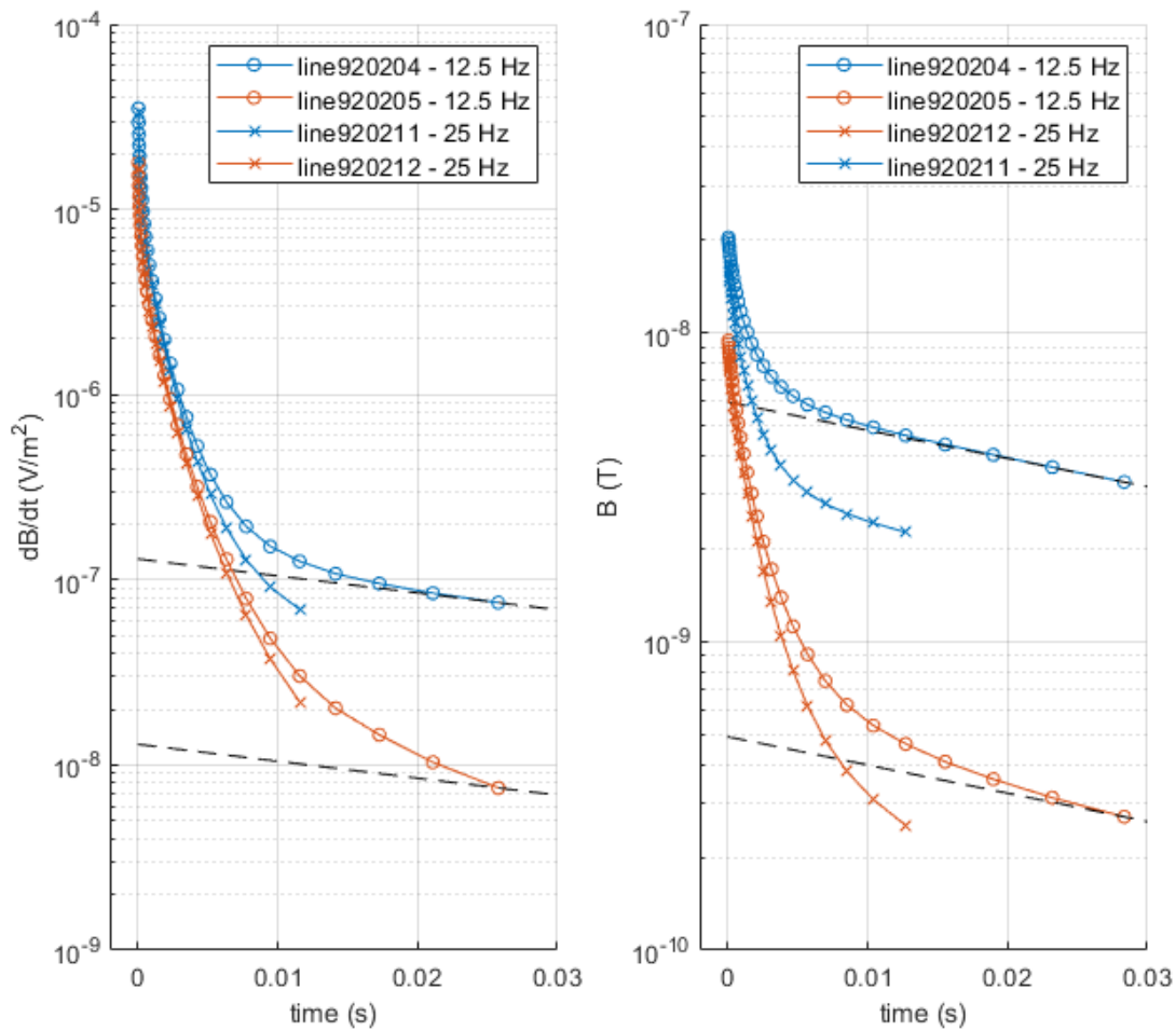
Figure 9: dB/dt and B -field responses measured over the wire loop target in 30 m (blue curves) and 50 m (red curves) with both 12.5 Hz and 25 Hz base frequencies. The dashed lines represent exponential functions with a time-constant of 47.5 ms.
