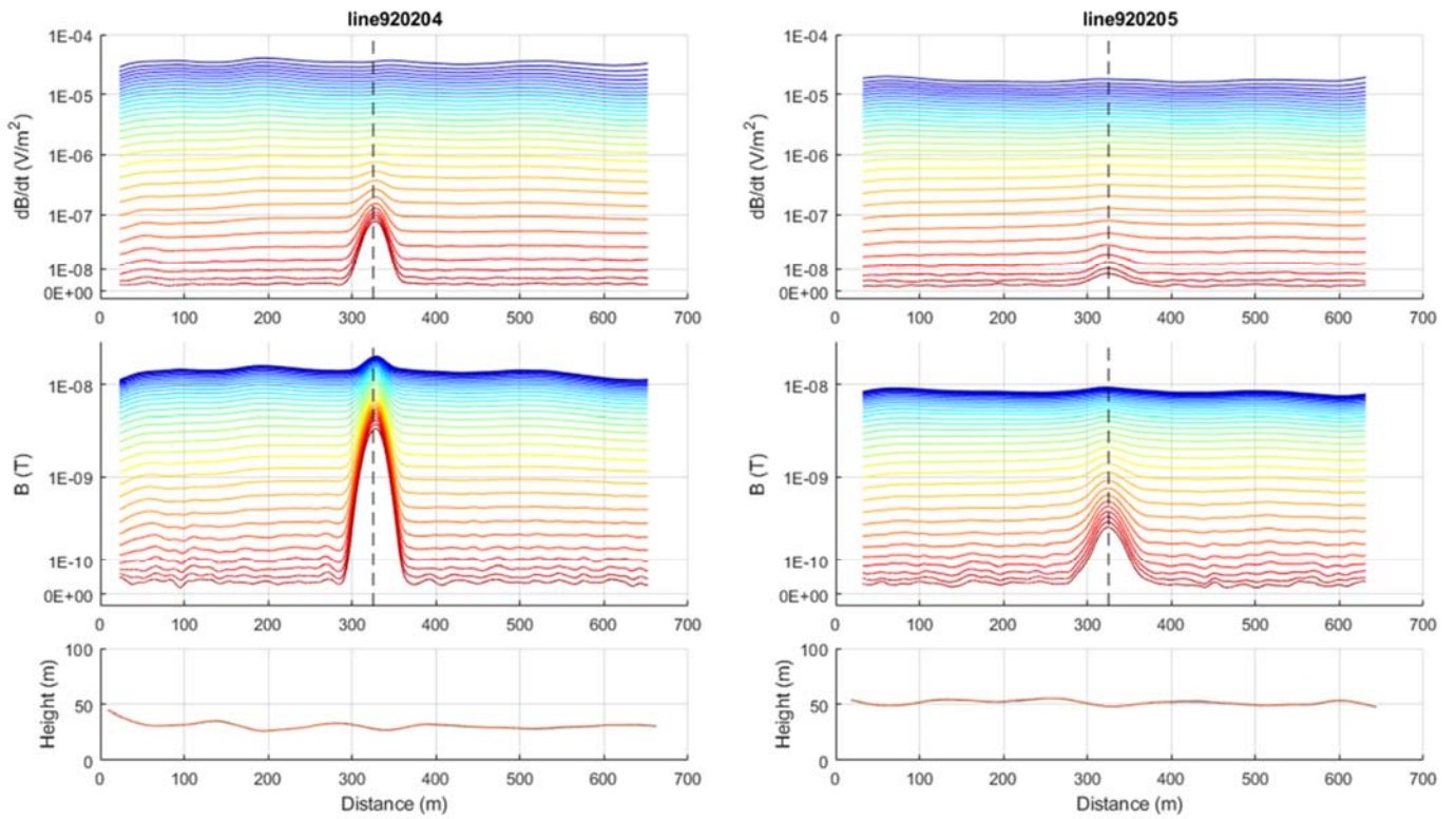
Figure 8: The left-hand and right-hand panels represent the wire loop target responses in 30 m and 50 m height above the target. The target responses are collected on profile lines 920204 and 920205 displayed in Figure 7.
