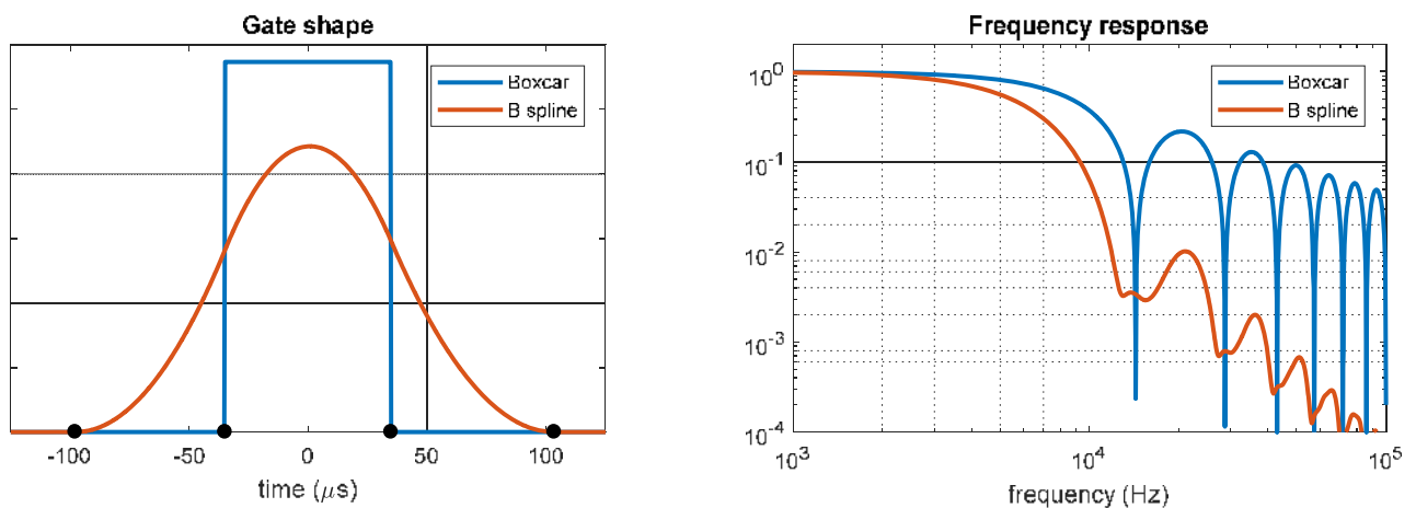
Figure 4: The left-hand panel shows a boxcar and a soft B-spline gate. The right-hand panel shows the frequency response for gate shapes to left.
