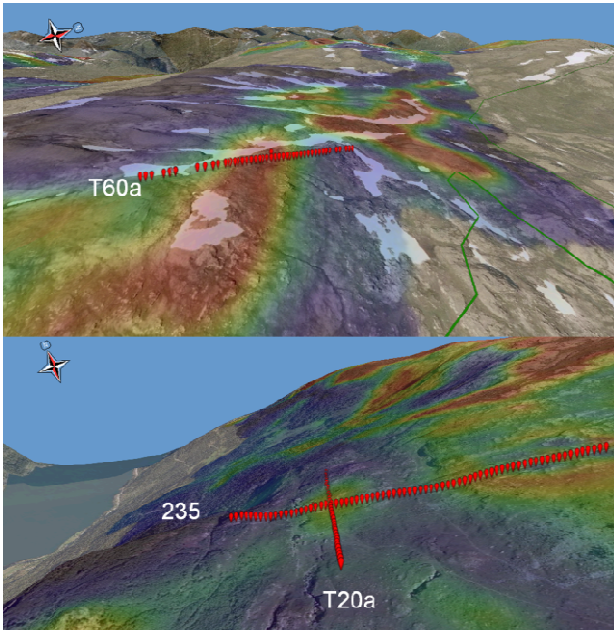
Figure 4: The three ERT profiles acquired in 2010. The colored background is the resistivity model acquired by the AEM survey in 2009. Upper panel shows line T60a in area A close to Viddalsdammen, lower panel shows intersecting profiles T20a and 235 in area B close to Joasete. Line T60a is 500m long striking NNE, line 235 700m ESE, and T20a 400 m NNE. Resistivity color scale according to Figure 2
