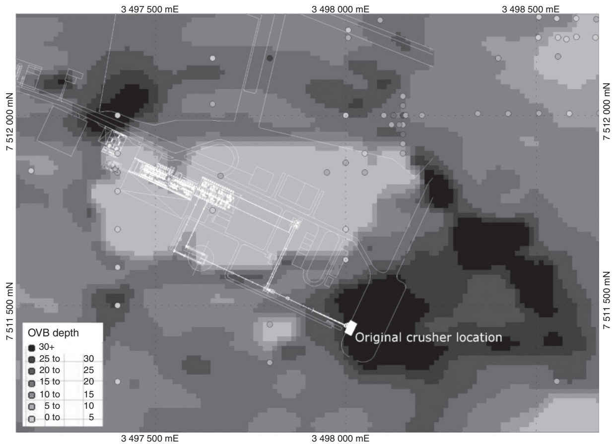
Fig. 3. Overburden (OVB) depth around the plant site derived from AEM data. Drillhole collars are coloured according to logged depth of overburden using the same scale as the EM-derived depth, where black is more than 30 m.
